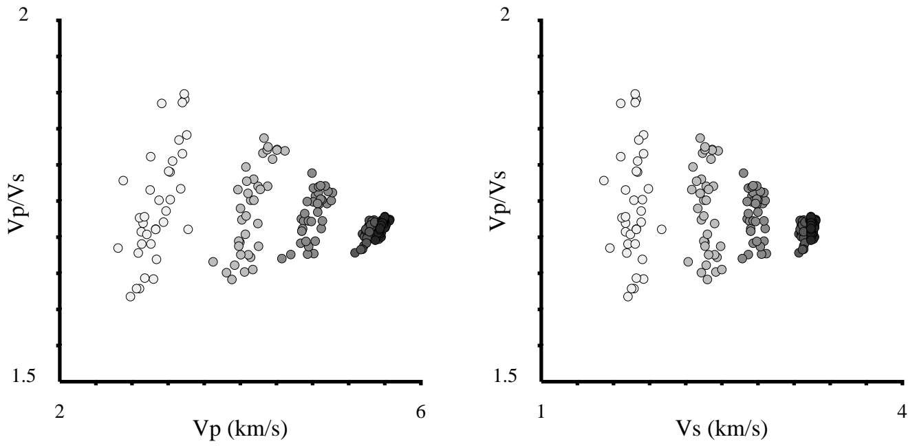
Figure 5: Model realization of the inversion data in Figure 1, assuming a homogeneous matrix, and a heterogeneous (random) distribution of K_f/G_f ranging from 2.5 to 4.0. The model is constrained to fit the V_s data exactly, and is used to predict V_p . In this case, the model fit improved when compared to Figure 3, but exhibits incorrect systematics between V_p , V_s , and V_p/V_s .
