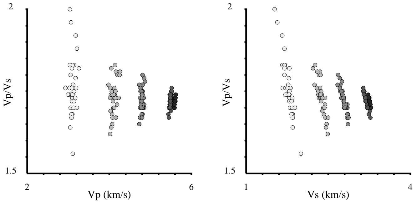
Figure 1: V_P and V_S versus V_P/V_S from a three dimensional velocity inversion at the Northwest Geysers [data from Romero et al. 1995 ]. Shading of symbols indicates depth, with darker shades reflecting increasing depth.
