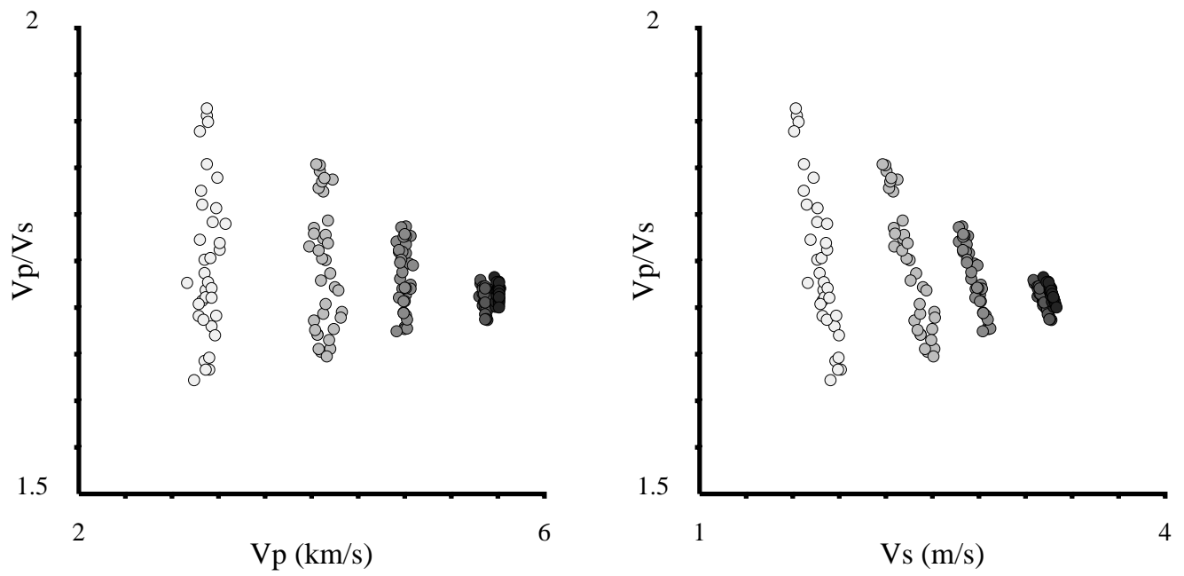
Figure 6: Model realization of the inversion data in Figure 1, with the same assumptions as in Figure 5, but this time constrained to fit the V_p data exactly, rather than V_s . In this case, the model exhibits the correct systematics between V_p , V_s , and V_p/V_s .
