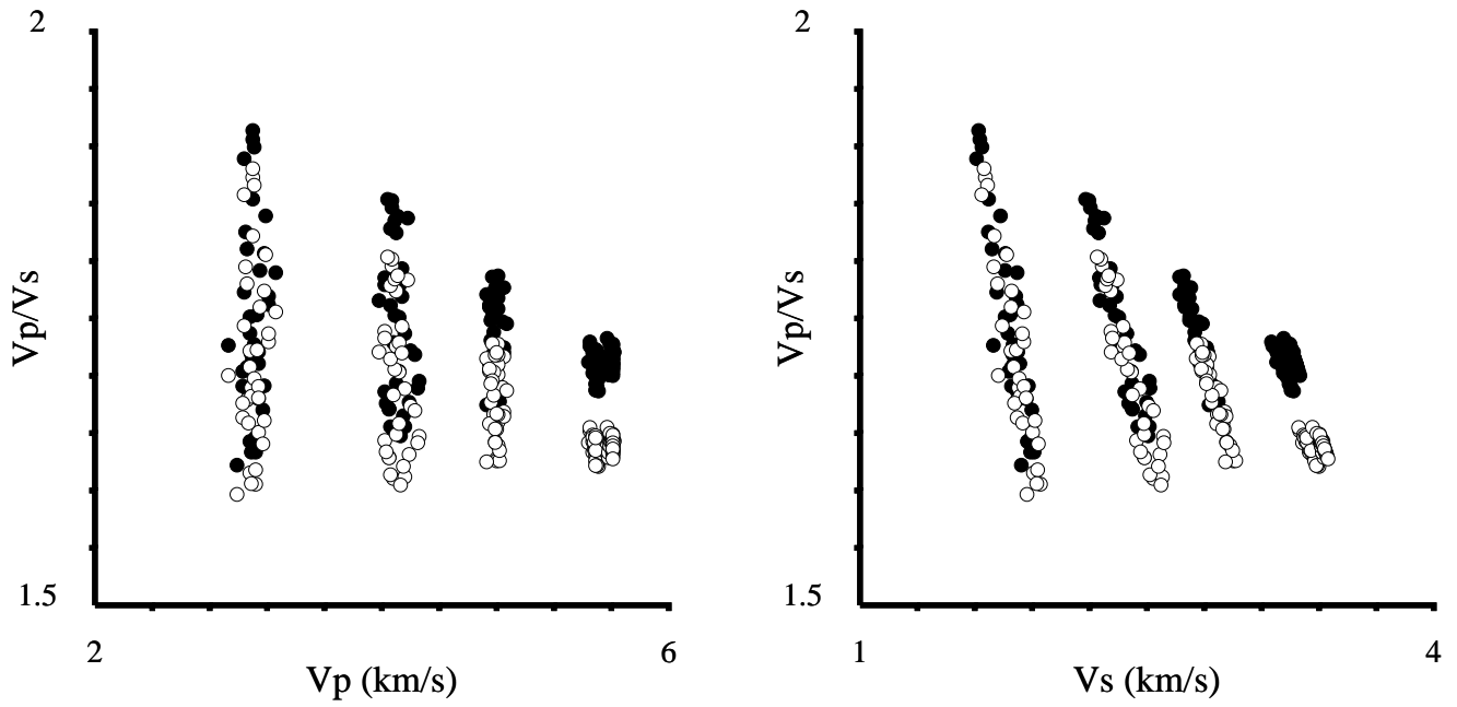
Figure 7: Stochastic model simulation similar to that in Figure 6, but assuming a matrix model with variable saturation. Open symbols indicate dry matrix and filled symbols indicate saturated matrix. Saturation effects in the matrix are clearly distinguishable at depth, but are hidden at the shallower levels by the considerable variation in V_p/V_s due to heterogeneity in K_f/G_f
