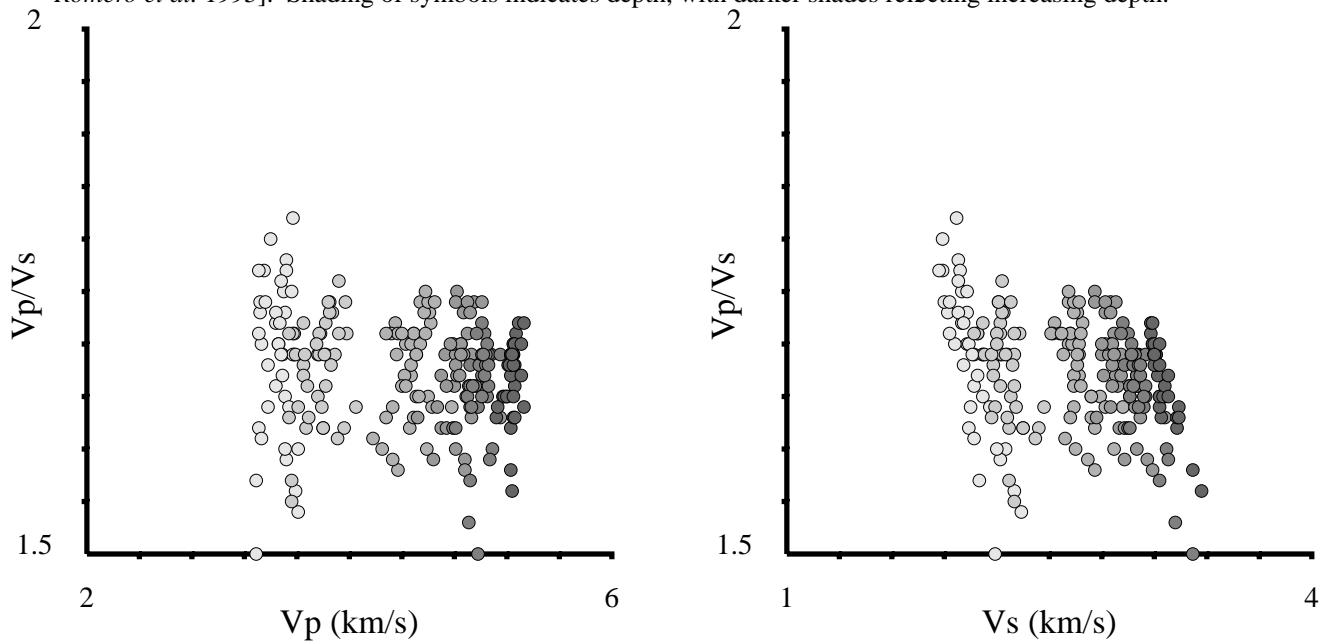
Figure 1: V_P and V_S versus V_P/V_S from a three dimensional velocity inversion at the Northwest Geysers [data from Romero et al. 1995 ]. Shading of symbols indicates depth, with darker shades reflecting increasing depth.
