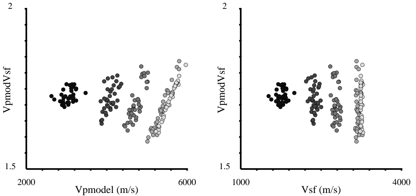
Figure 3: V_p and V_s versus V_p/V_s from laboratory measurements on matrix material from The Geysers. Open symbols indicate dry matrix and filled symbols indicate saturated matrix.
