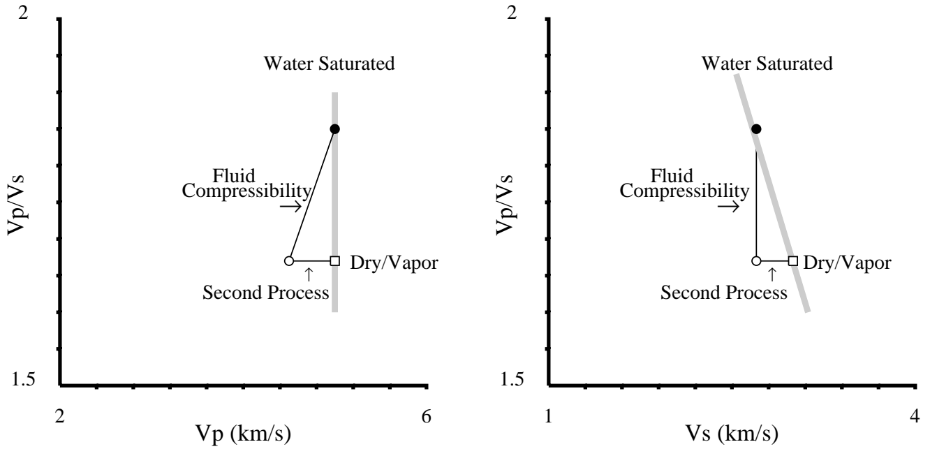
Figure 8: Schematic illustration of the general physical interpretation of the field seismic observations. The solid dot indicates the velocity properties of water saturated reservoir. Upon drying, two effects are super-imposed. First, the increase in fluid compressibility decreases the effective bulk modulus, thus decreasing V_p . It is assumed that changes in effective density are negligible and that fluid compressibility does not effect the shear modulus (and thus shear velocity). Second, upon drying a second process occurs, which acts to increase both V_p and V_s , without influencing V_p/V_s . In the context of the shear weakening hypothesis, the second process is the hardening of the shear modulus upon drying, while in the context of the pore pressure reduction hypothesis, this process is the effect of increasing effective stress with depletion.
